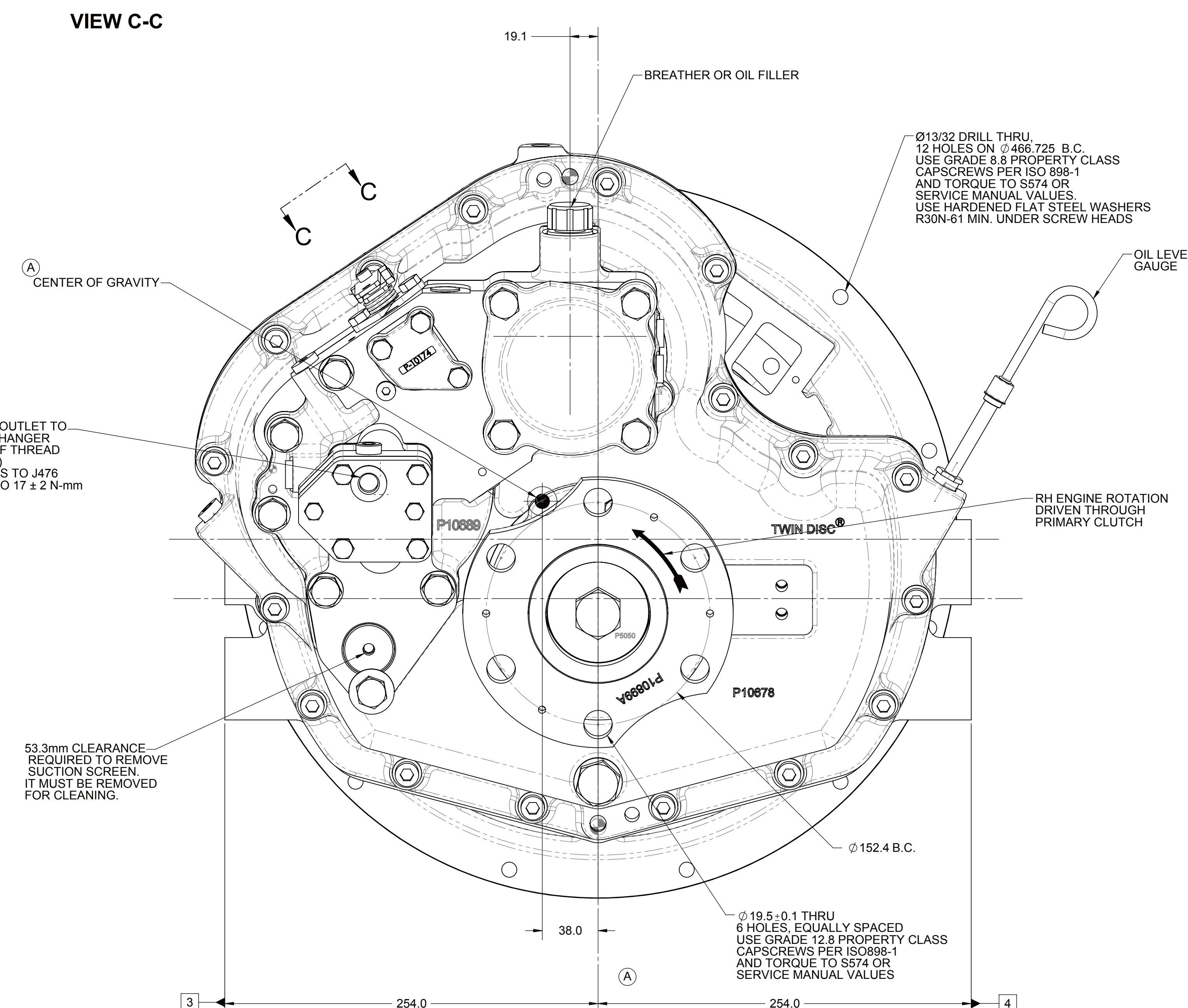
VIEW C-C
