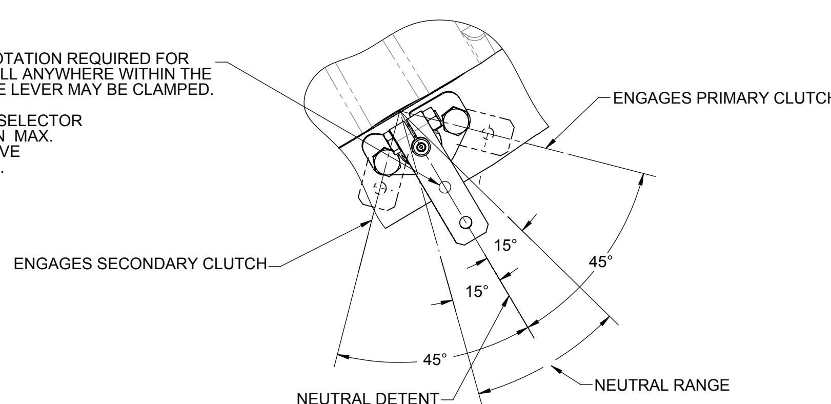
VIEW C-C
