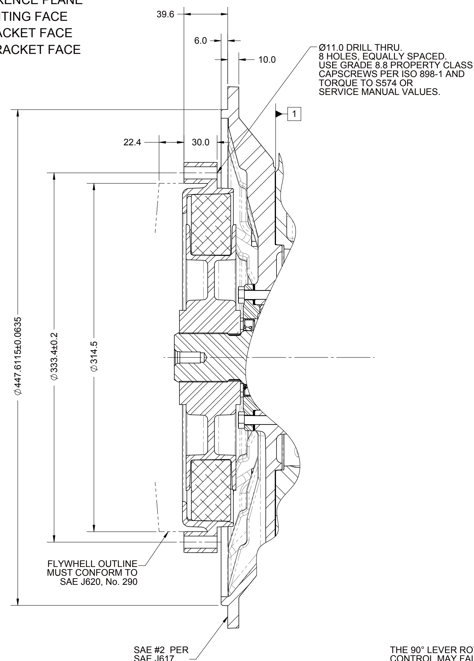
SECTION B-B
