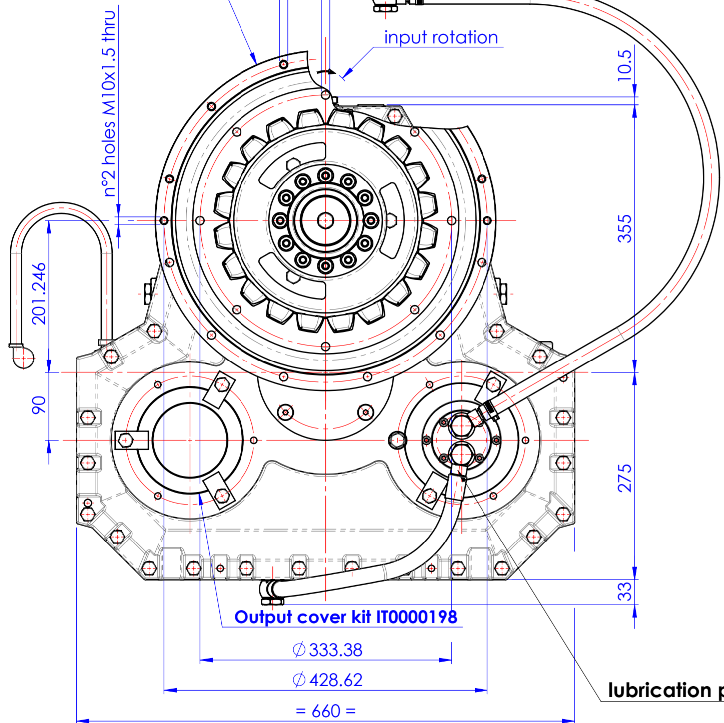
lateral input assy IT1071135 housing SAE 3 flywheel 11,5"
