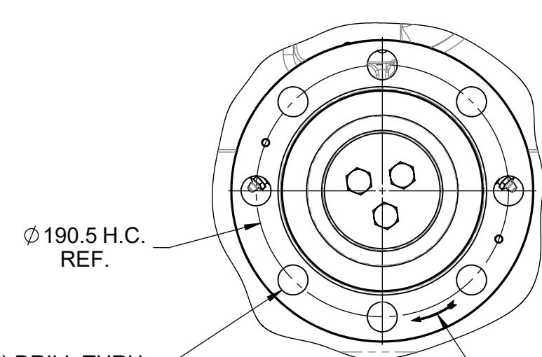
VIEW B-B
