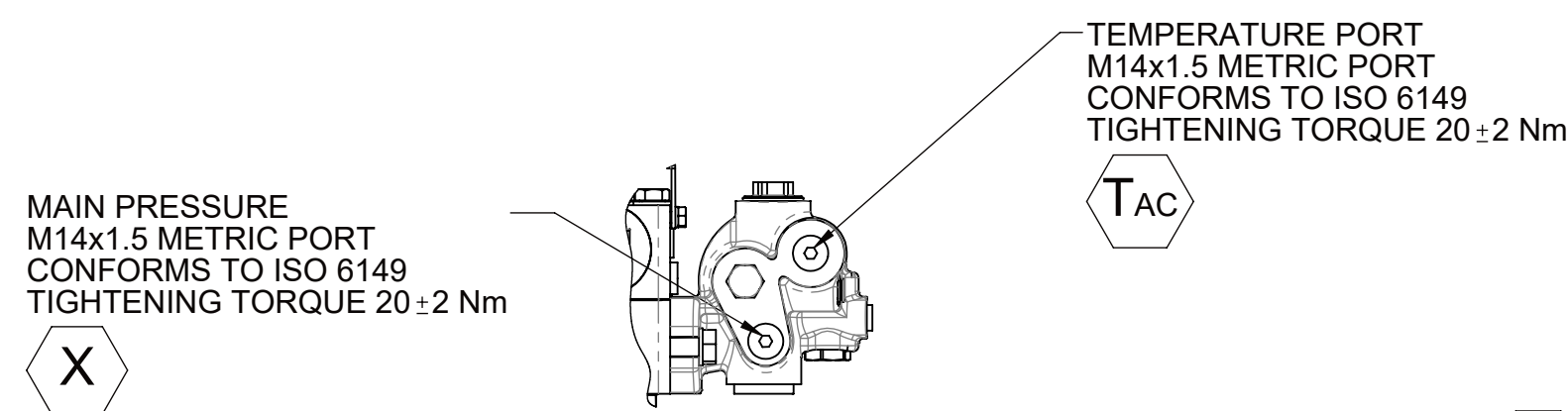
VIEW C-C
