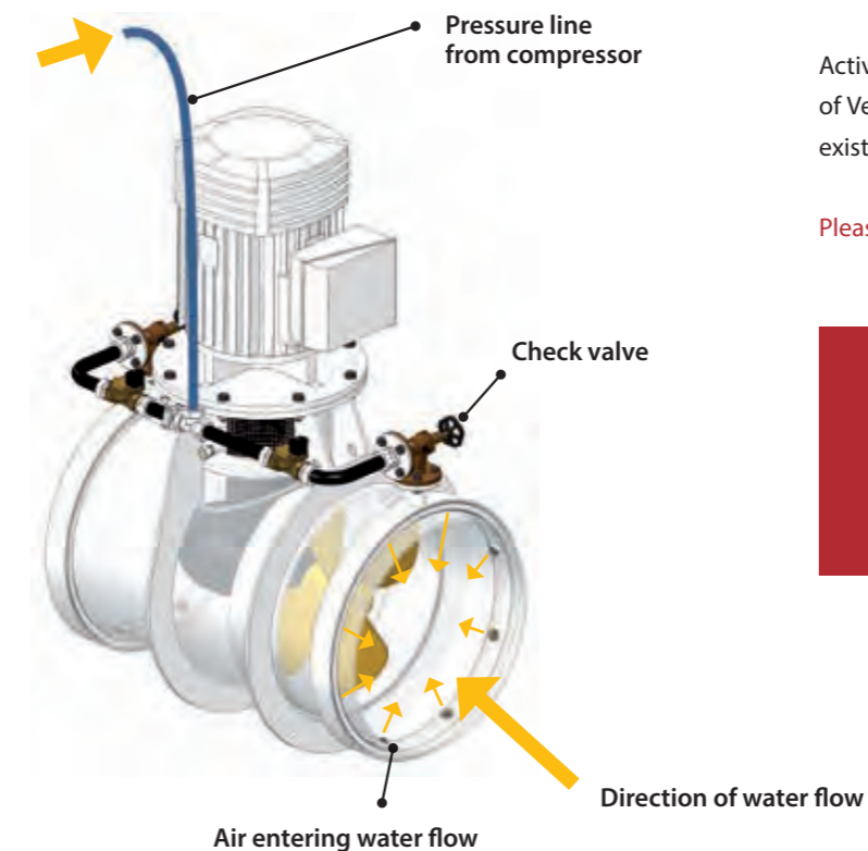
System activated - compressed air injected into tunnel's water flow
