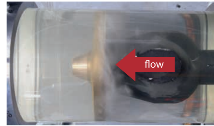
Thruster producing cavitation (imploding vacuum bubbles) - ANS off
