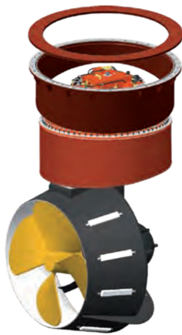
Rigid bolted suspension
